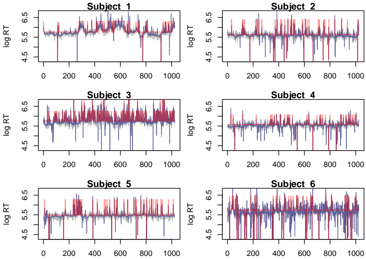
Figure 12: Observed log RTs for the Wagenmakers data (gray lines) and posterior predictive median log RTs under the HMM (red lines) and wavelet model (navy lines).
