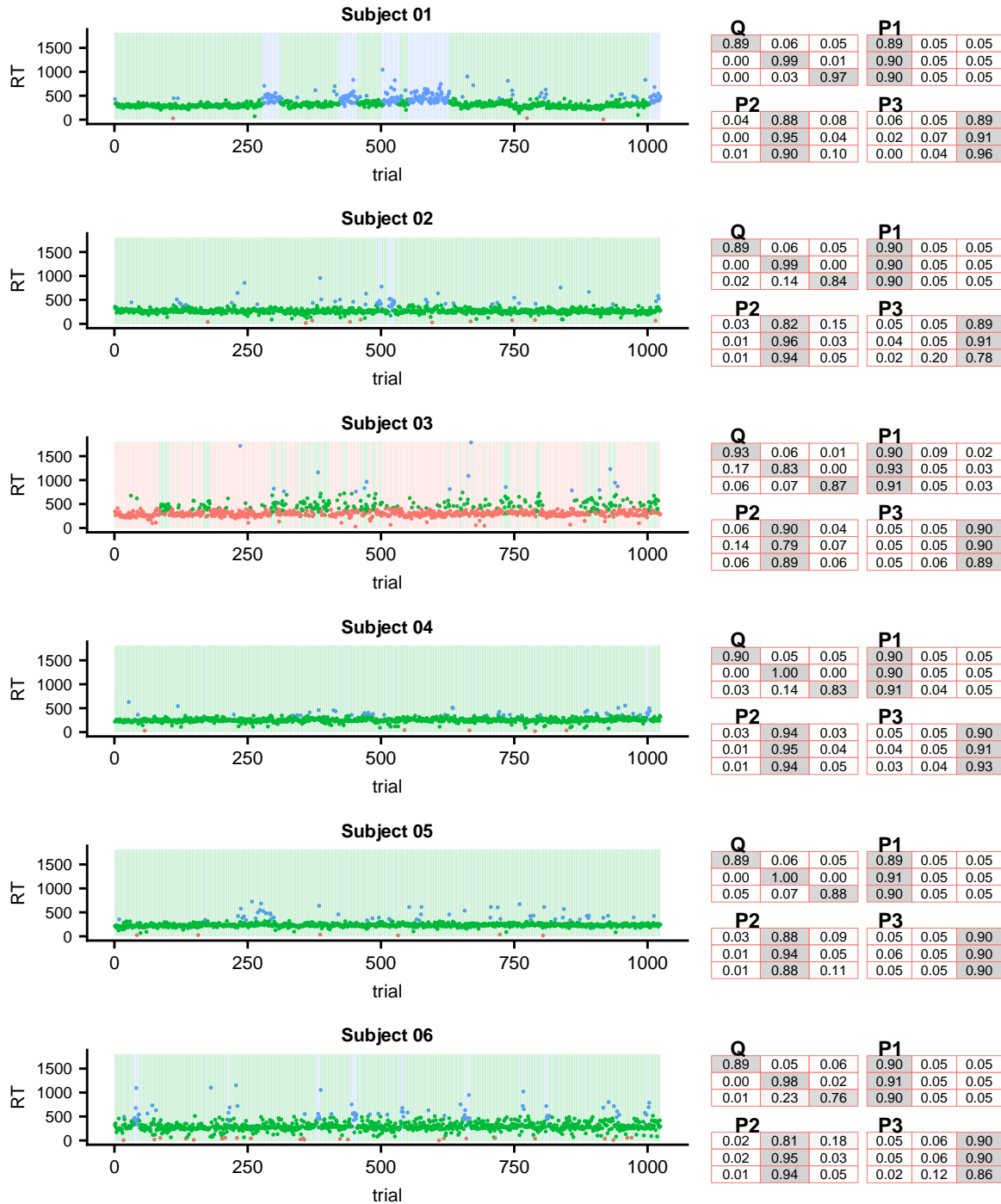
Figure 11: Estimated environments and response modes and posterior expected TPMs for the Wagenmakers data.
