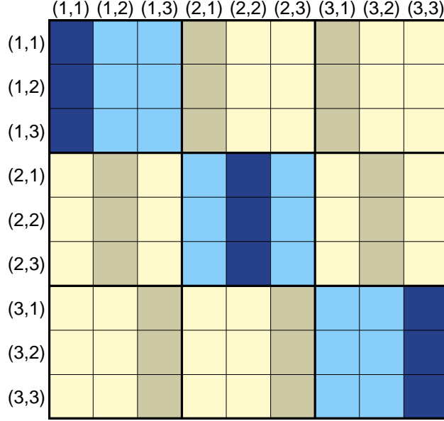
Figure 2: Qualitative structure of the expected prior transition probability matrix for the hidden states. The state corresponding to environment e and response mode r is labeled (e, r) . Blue represents large probabilities and tan represents small probabilities, with darker shades representing larger probabilities within either color.
