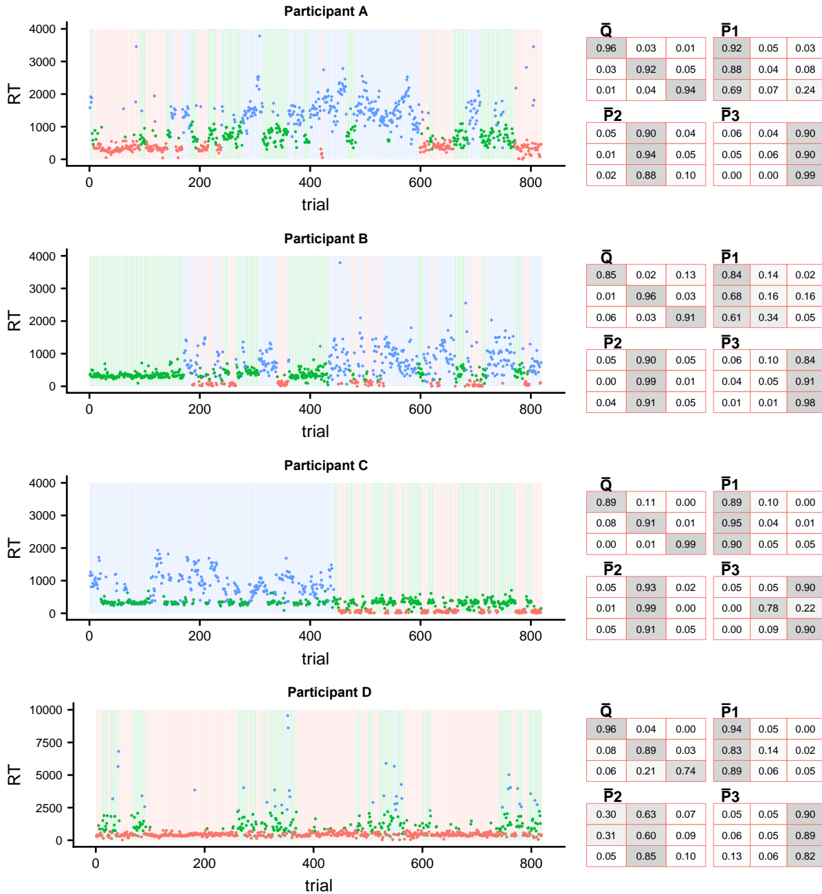
Figure 8: RT sequences for the selected participants. The plot background color corresponds to the estimated environment and the plotting color corresponds to the estimated response mode. The y-axis value is the observed RT at that trial. The matrices \bar{Q}^{(i)} and \bar{P}^{(i,e)} are shown to the right with darker shades of gray denoting higher values of the probabilities.
