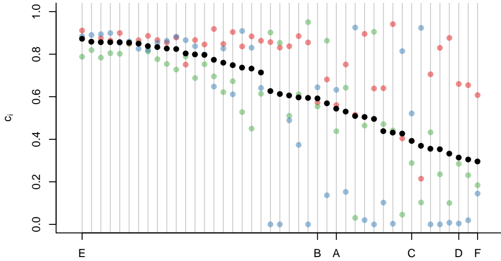
Figure 9: Values of the within-environment and overall similarities, c_{i1} , c_{i2} , c_{i3} , and c_i , shown for each participant in red, green, blue, and black, respectively. The participants are shown in order of descending c_i to improve readability.
